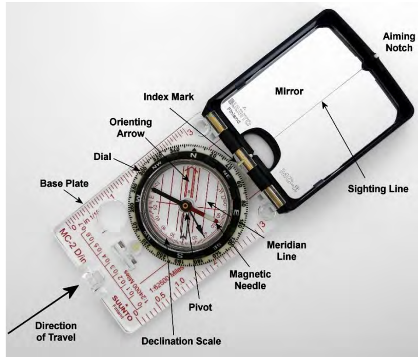
Figure 7: Principal parts of the Suunto MC-2 D/in
