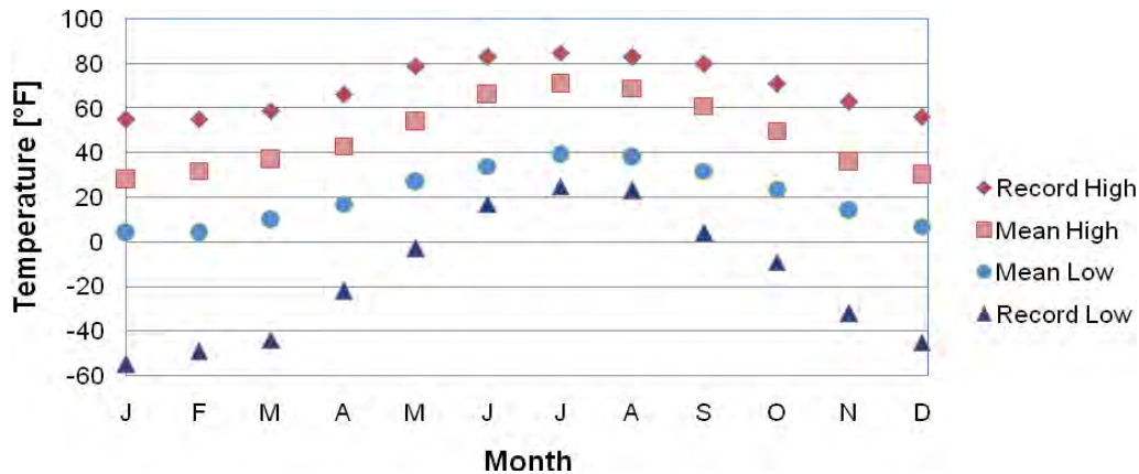
Figure 2: Temperatures in Leadville, CO
