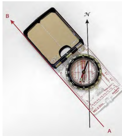
Figure 10: Measuring the bearing from point A to point B
