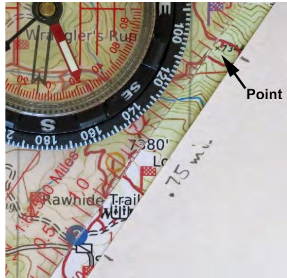
Figure 12: Plotting the position of a point on the map 0.75 miles from the kiosk on a true bearing of 035°
