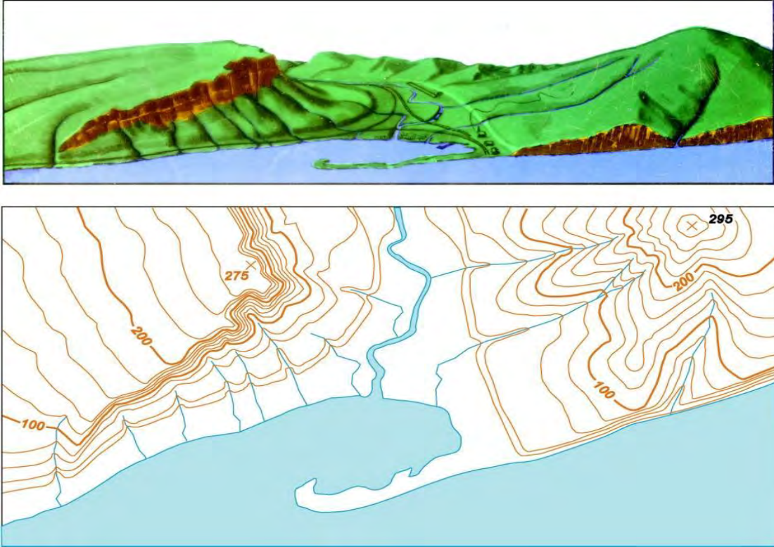
Figure 4: Perspective drawing of a landscape and contour map of the same landscape. Contour interval is 20 feet.
